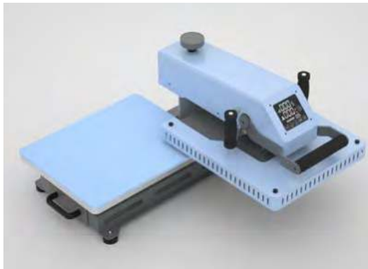
Swing-away Design
